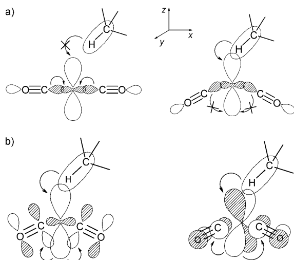
Figure 2. Critical orbital interactions responsible for the anagostic bonding. a) Bending-induced changes in the \sigma system. In the linear complex (left), the CO \rightarrow Rh \sigma donation hinders the anagostic interaction by hampering the \sigma_{\text{C-H}} \rightarrow Rh electron donation; in the bent complex (right) the CO \rightarrow Rh \sigma donation is itself hampered, thereby allowing the \sigma_{\text{C-H}} \rightarrow Rh electron donation. b) Bending-induced, anagostic-enhancing interactions in the \pi system (left: d_{z^2} \rightarrow \pi^* , right: d_{yz} \rightarrow \pi^* ).
